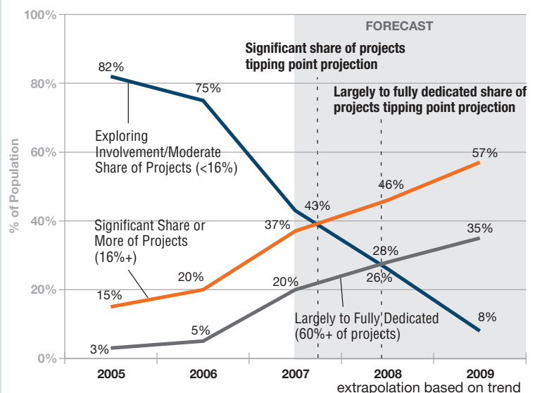
“Tipping Point” Analysis
