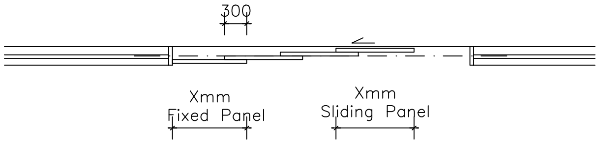
PLAN VIEW
