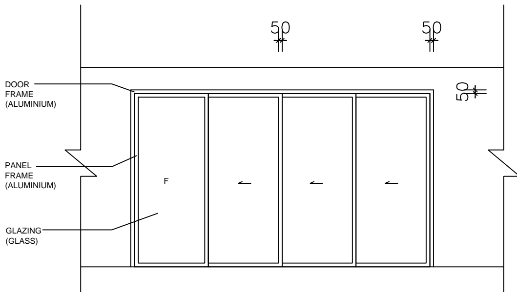
ELEVATION VIEW
