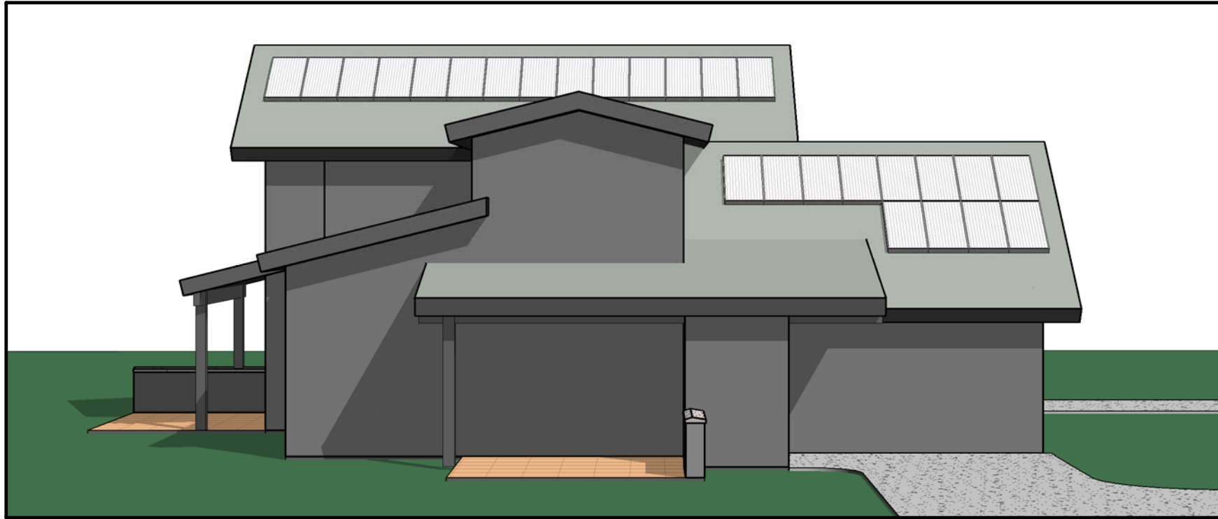
south elevation
