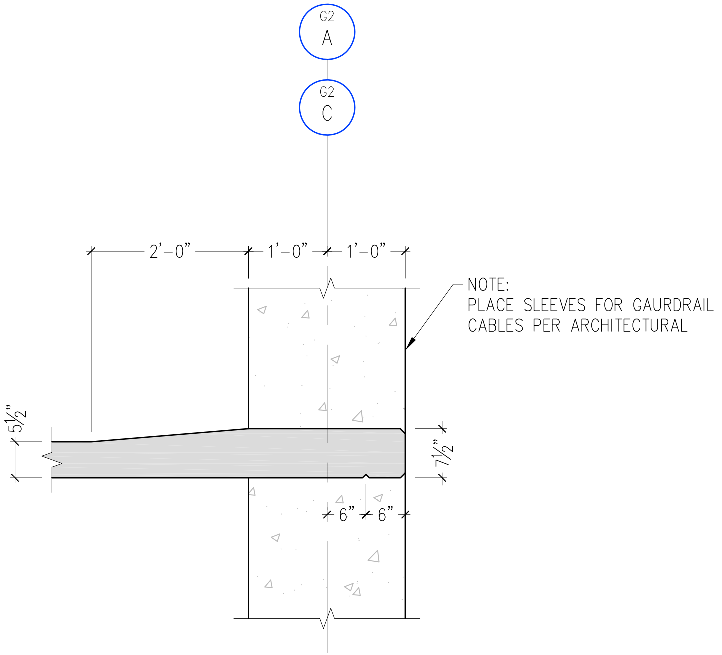
10 TYPICAL SLAB EDGE AT "A" AND "C" 1/2" = 1'-0"
