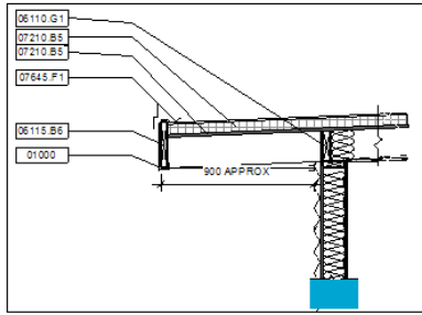
Roof Overhang Detail - 2 Keynotes 1:20
