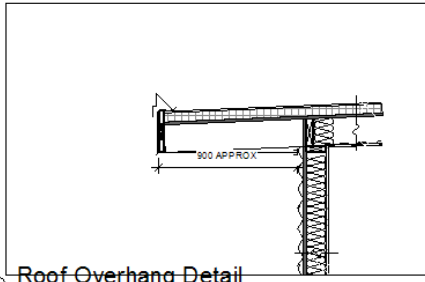
1 Roof Overhang Detail 1:20
