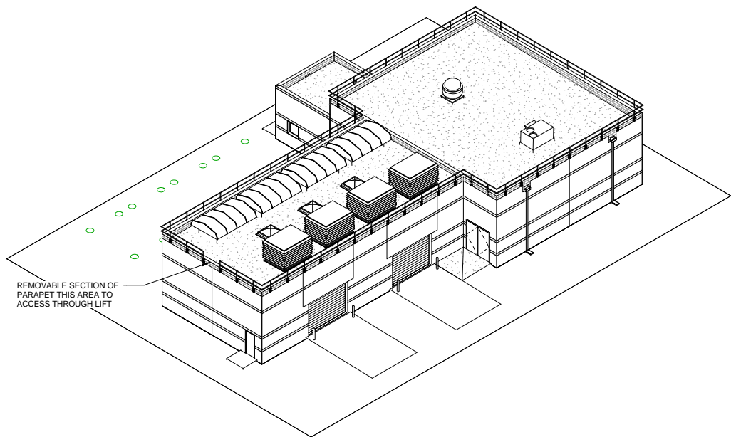
③ WEST VIEW
