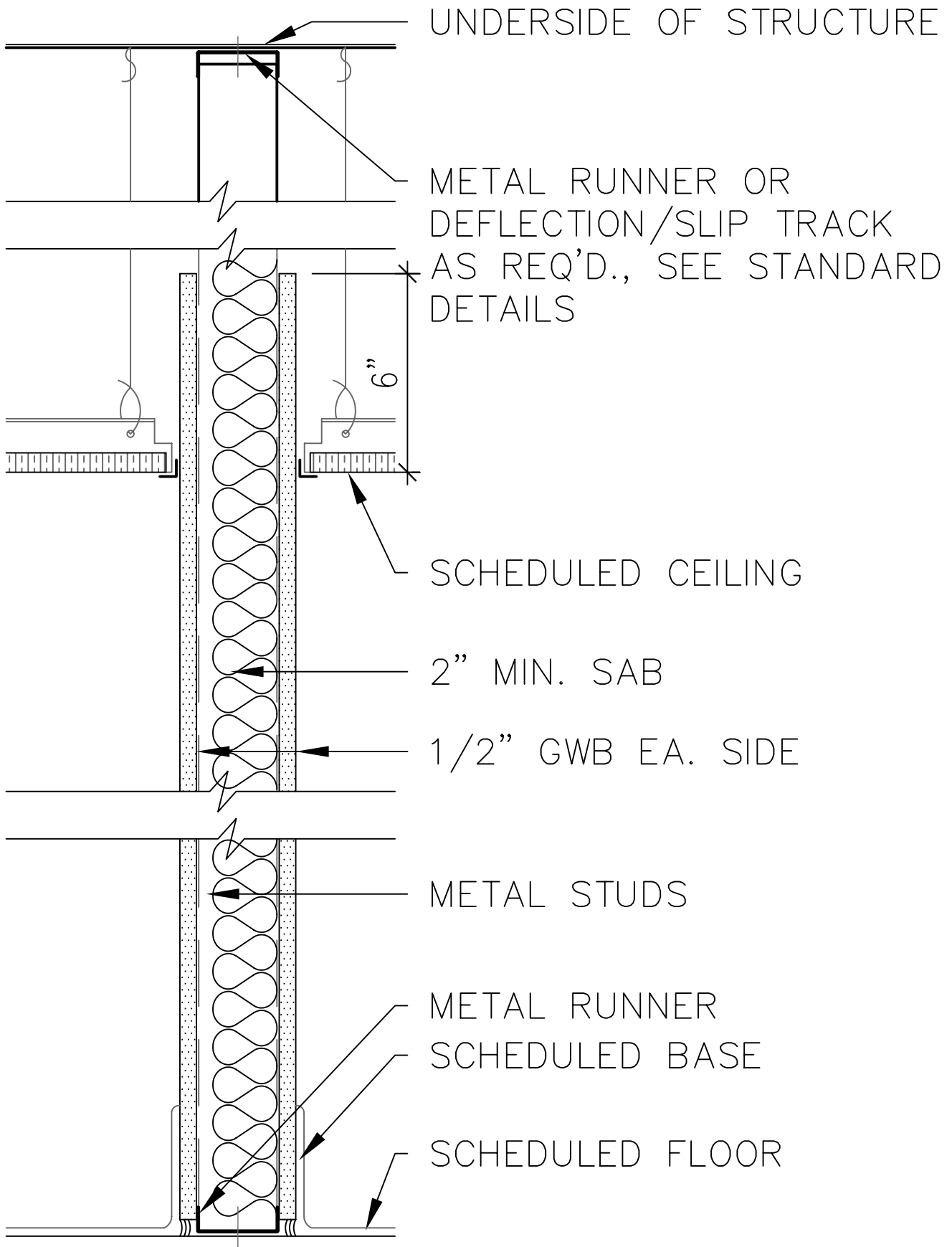
SECTION
