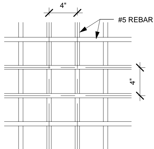
TOP VIEW DETAILS OF TYPICAL REBAR GRID LAYOUT
