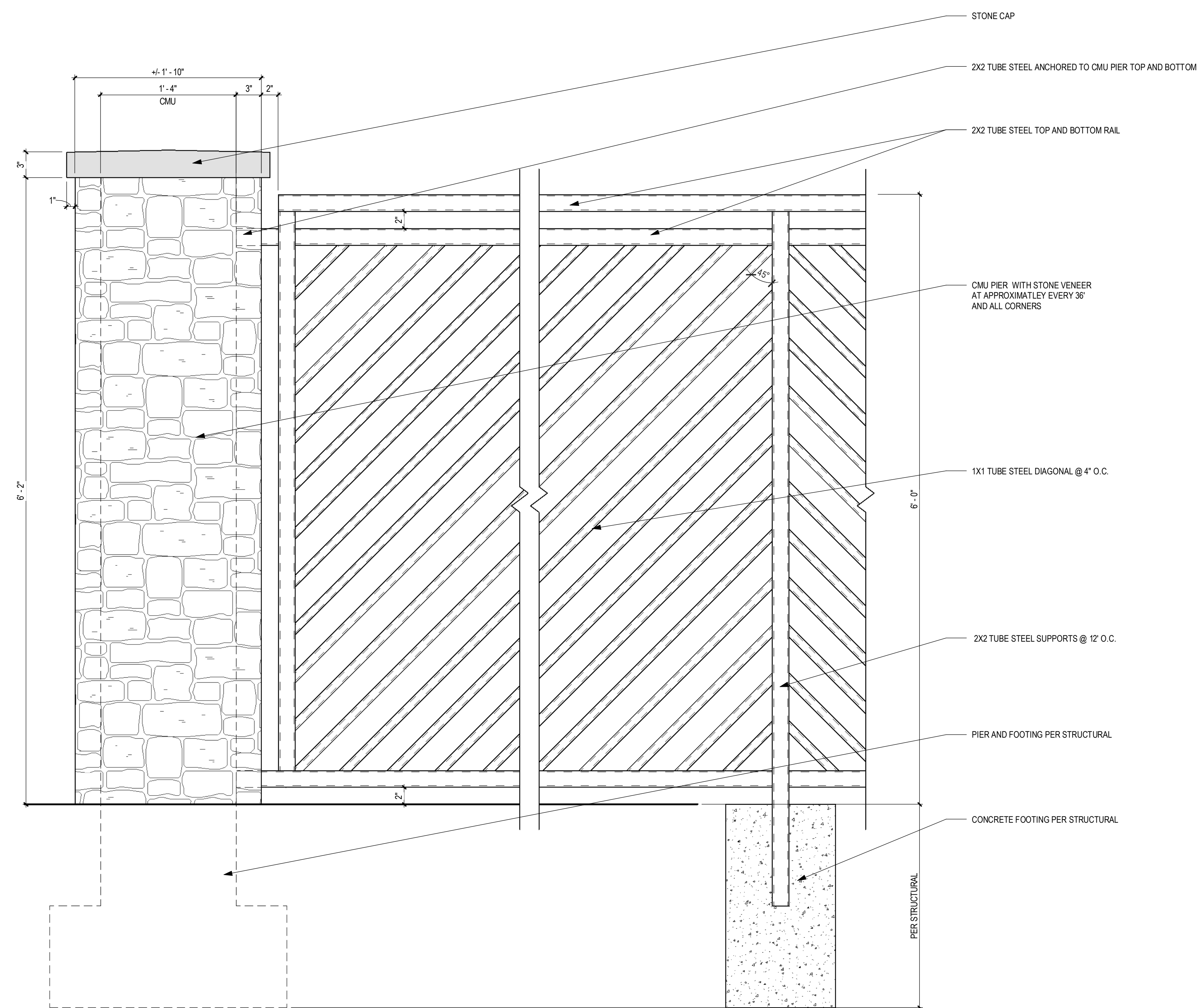
1 FENCE C PLAN SCALE: 1/12" = 1'-0"
