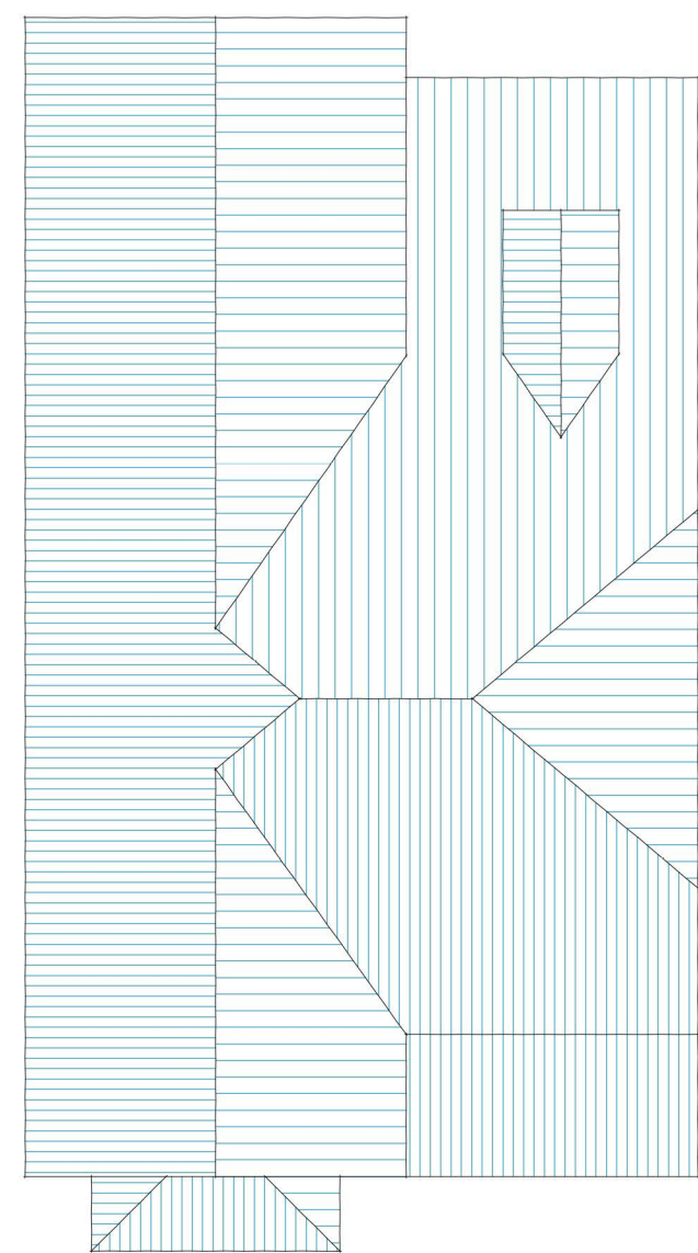
ROOF PLAN
