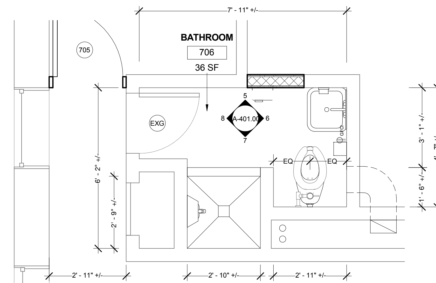
10 BATHROOM 706 PLAN 1/2" = 1'-0"
