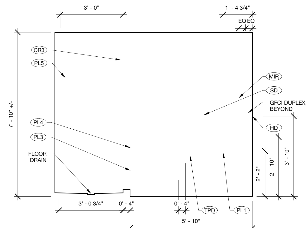
1 BATHROOM 703 INT ELEVATION (N) 1/2" = 1'-0"
