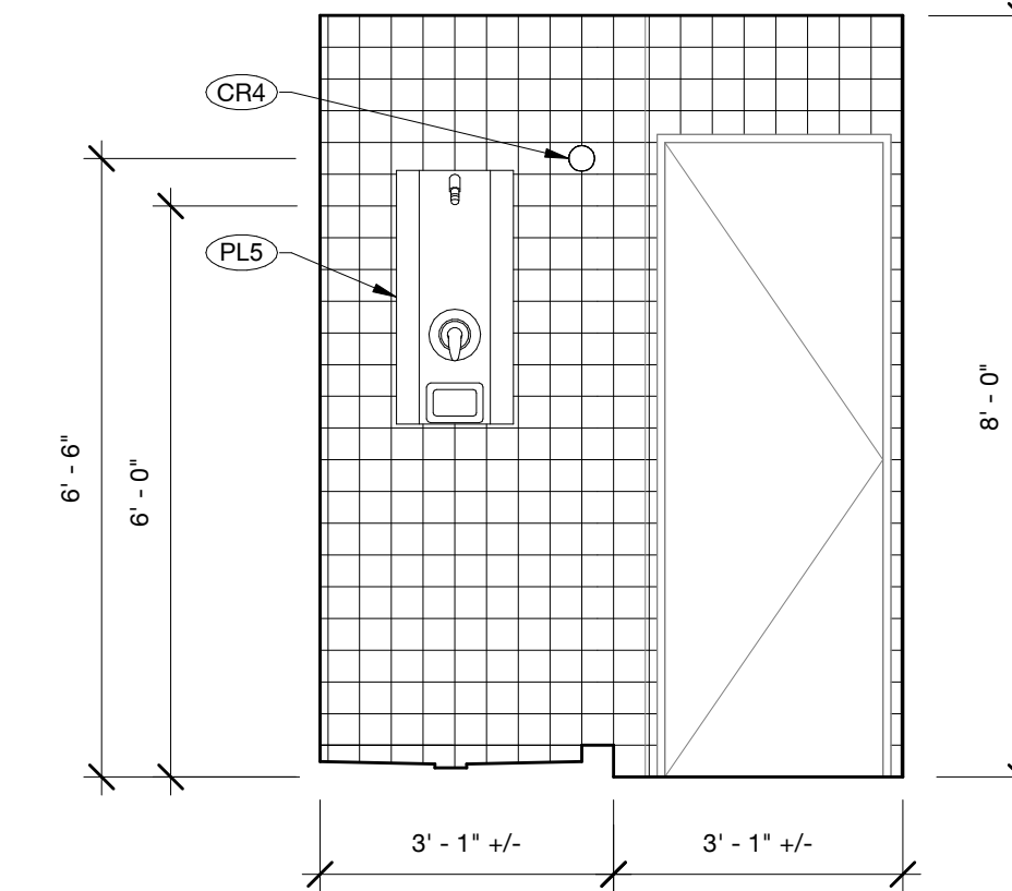
8 BATHROOM 706 INT ELEVATION (W) 1/2" = 1'-0"
