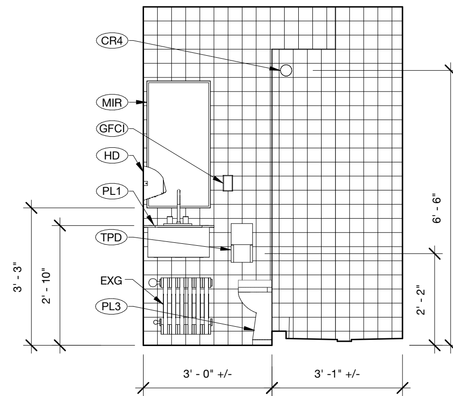
6 BATHROOM 706 INT ELEVATION (E) 1/2" = 1'-0"
