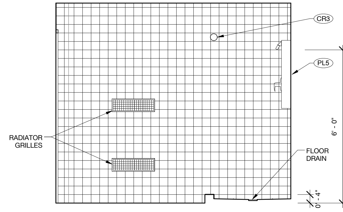
3 BATHROOM 703 INT ELEVATION (S) 1/2" = 1'-0"
