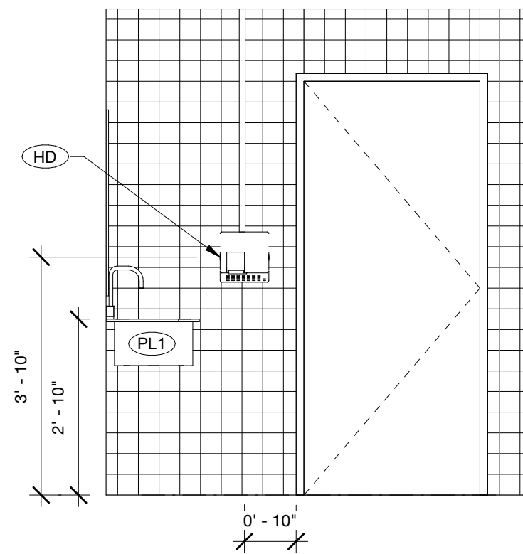
2 BATHROOM 703 INT ELEVATION (E) 1/2" = 1'-0"
