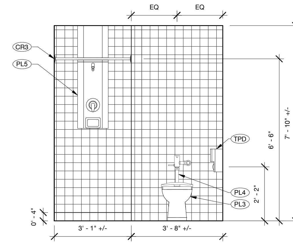
4 BATHROOM 703 INT ELEVATION (W) 1/2" = 1'-0"
