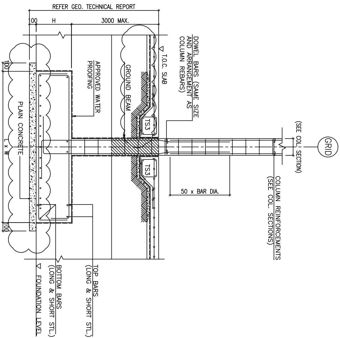
1 TYPICAL FOOTING DETAIL SCALE N.T.S.
